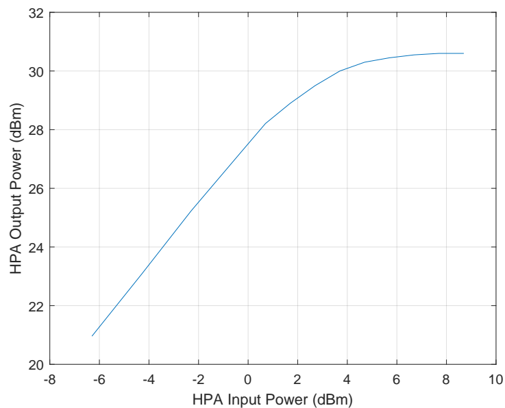
Figure 2-7: AM/AM characteristic of the HPA
